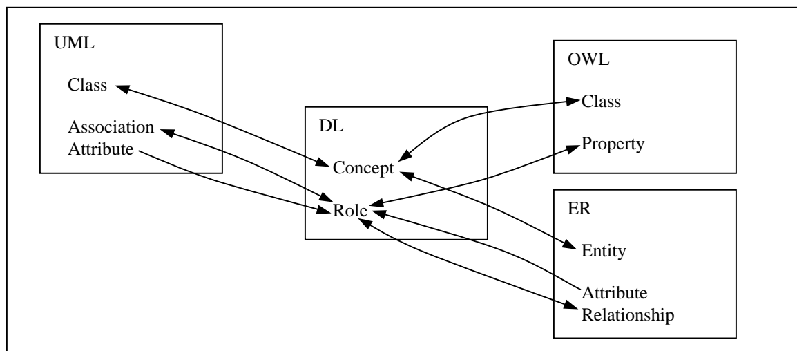
Figure 1: Naïve mappings between UML, DL, OWL and ER.
