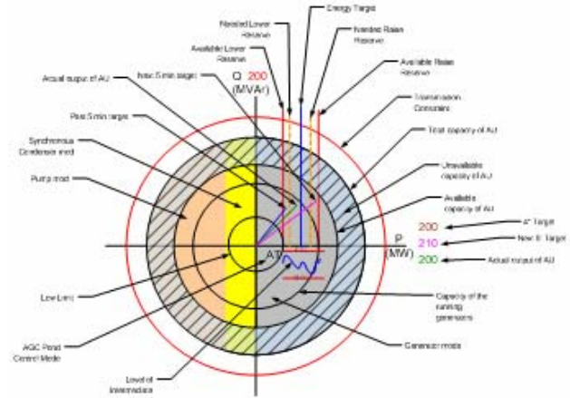
Figure 4. Complex power display
