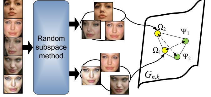
Fig. 1: Graphical interpretation of the proposed method. For any image-set, a random ensemble of subspaces ( \Omega_i ) and their furthest subspaces ( \Psi_i ) are generated and used for classification.
