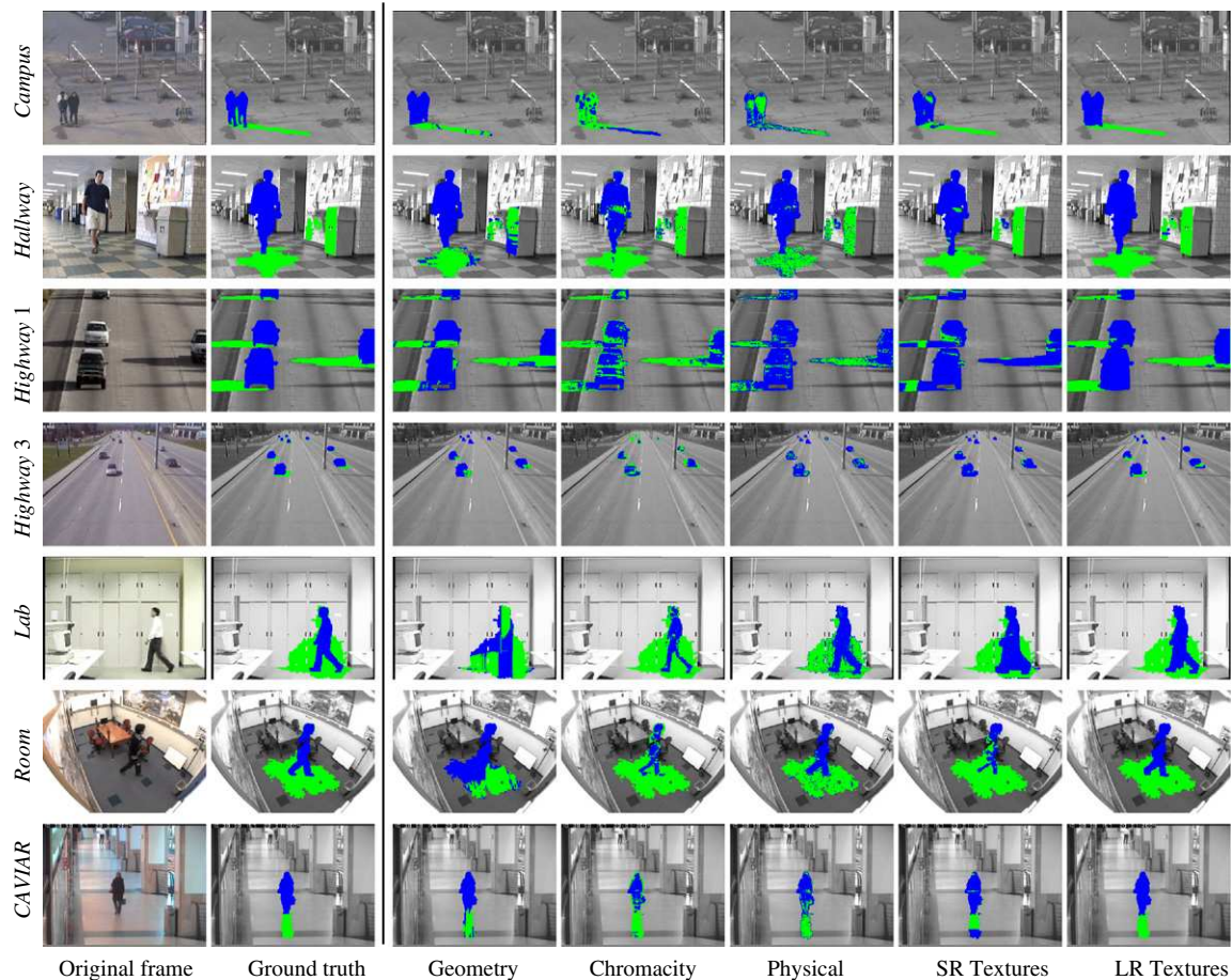
Fig. 5. Qualitative shadow detection results. The first column shows an example frame for each sequence. The second column show the expected results where object pixels are marked in blue and shadow pixels are marked in green. The remaining columns show the observed results for each method. The geometry-based method works well for long shadows with a well defined orientation ( Campus example) but does not work well for spread shadows ( Lab example). Both the chromacity-based and physical methods are affected by pixel-level noise, and fail when objects are darker and have similar colours to the background ( Campus example), although the physical method adapts better to the different scenes. The small region (SR) texture-based method fails for pixels located in non-textured neighbourhoods ( Highway 1 example). The large region (LR) texture-based method works reasonably well in all cases. (For interpretation of the references to colour in this figure legend, the reader is referred to the web version of this article.)
