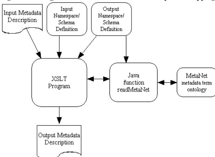
Figure 4: Program Flow for Metadata Description Mappings
