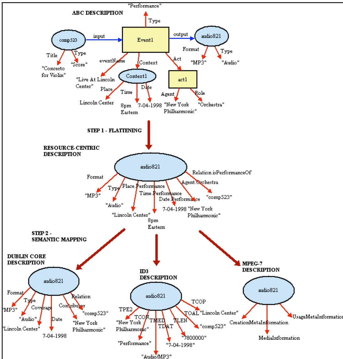
Figure 2: Transformation from the ABC Event-aware Model to 3 Different Resource-centric Models
