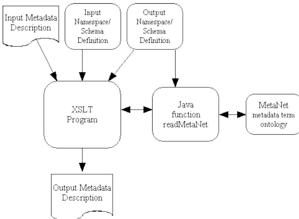
Figure 4 - Program Flow for Metadata Description Mappings
