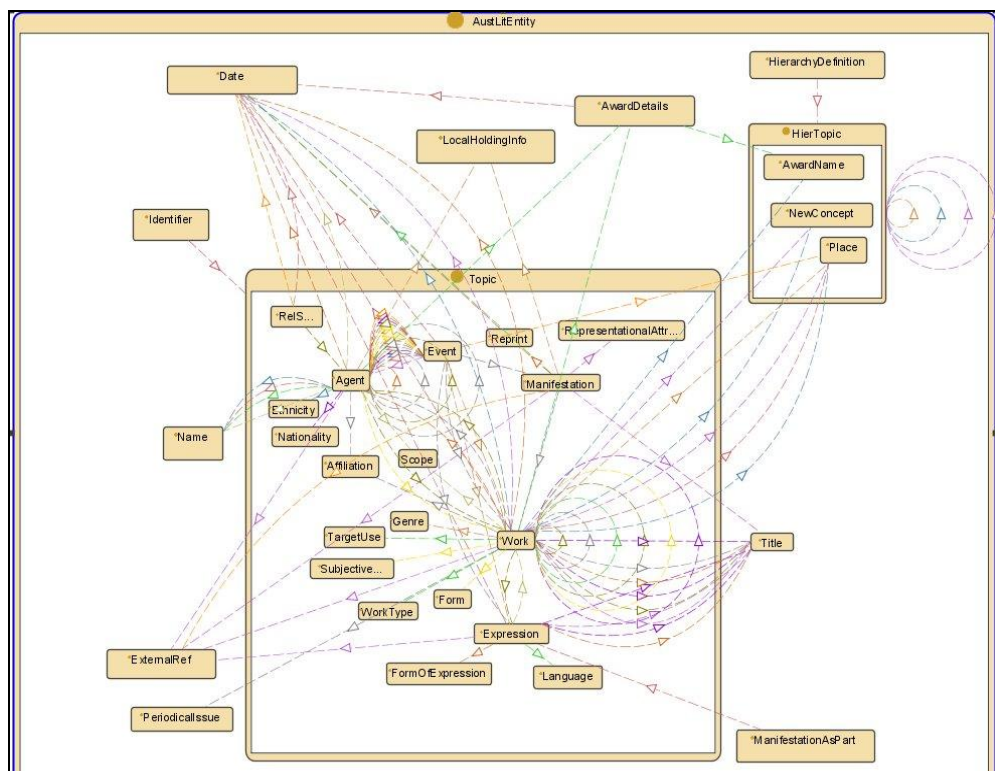
Fig.3. A subset of the OWL object properties from the AustLit Ontology
