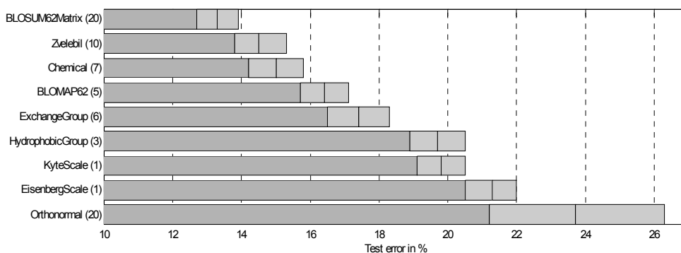
Figure 4. Mean test error and 95%-confidence intervals for the Single Layer Perceptron over all data sets. Lower value is better. The numbers in brackets indicate the dimensionality of the encoding.
