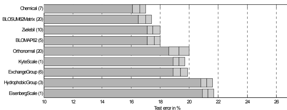
Figure 2. Mean test error and 95%-confidence intervals for all encoding over all classifiers and data sets. Lower value is better. The numbers in brackets indicate the dimensionality of the encoding.
