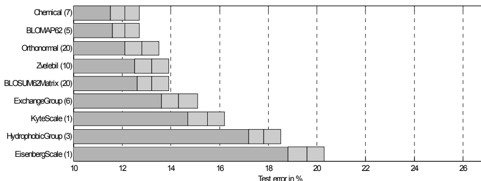
Figure 3. Mean test error and 95%-confidence intervals for the Naïve Bayes classifier over all data sets. Lower value is better. The numbers in brackets indicate the dimensionality of the encoding.
