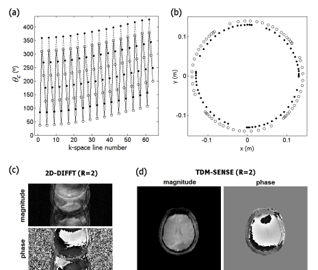
Fig. 3. Comparison of inverse FFT and TDM-SENSE 128 \times 128 image reconstruction with R=2 . FLASH sequence: TR=100 \text{ ms} , TE=10.16 \text{ ms} , FOV=35 \times 35 \text{ cm} , 512 frequency and 64 phase readouts, ST=5 \text{ mm} , FA=30^\circ , b_1(t)=\text{hermite pulse} , T_{acq}=10.24 \text{ ms} . (a) Measured angular coil positions when the RF coil was rotating at about 82.8 \text{ rad s}^{-1} , where circles and dots indicate start and end of the signal acquisition; (b) Distribution of angular positions visited by the RF coil (according to measurements in (a)); (c) and (d) show magnitude and phase plots of the inverse FFT and TDM-SENSE reconstructed brain image, respectively.
