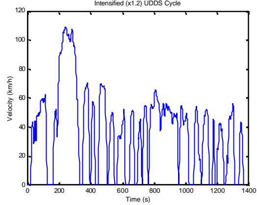
Figure 2: The intensified UDDS cycle
