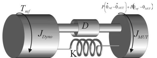
Figure 2: Spring-damper model.
