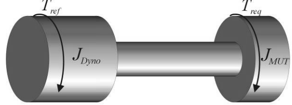
Figure 1: Rigid mass model.
